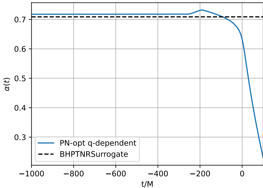
PN-opt q-dependent Agentic fit ( q = 3 )
