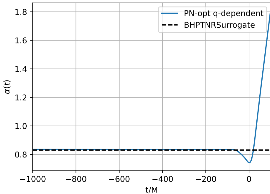
PN-opt q-dependent Agentic fit ( q = 6 )
