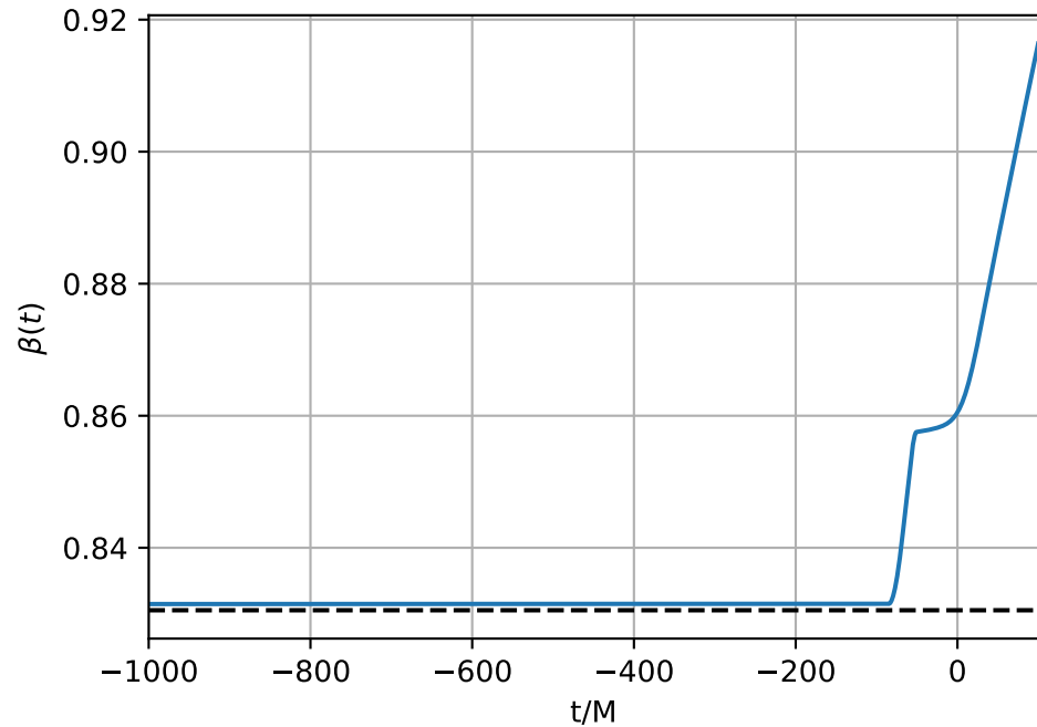
PN-opt q-dependent Agentic fit ( q = 6 )
