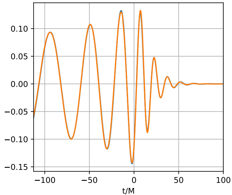
PN-opt q-dependent Agentic fit ( q = 8 ); \text{mathcal{E}} = 0.000107
