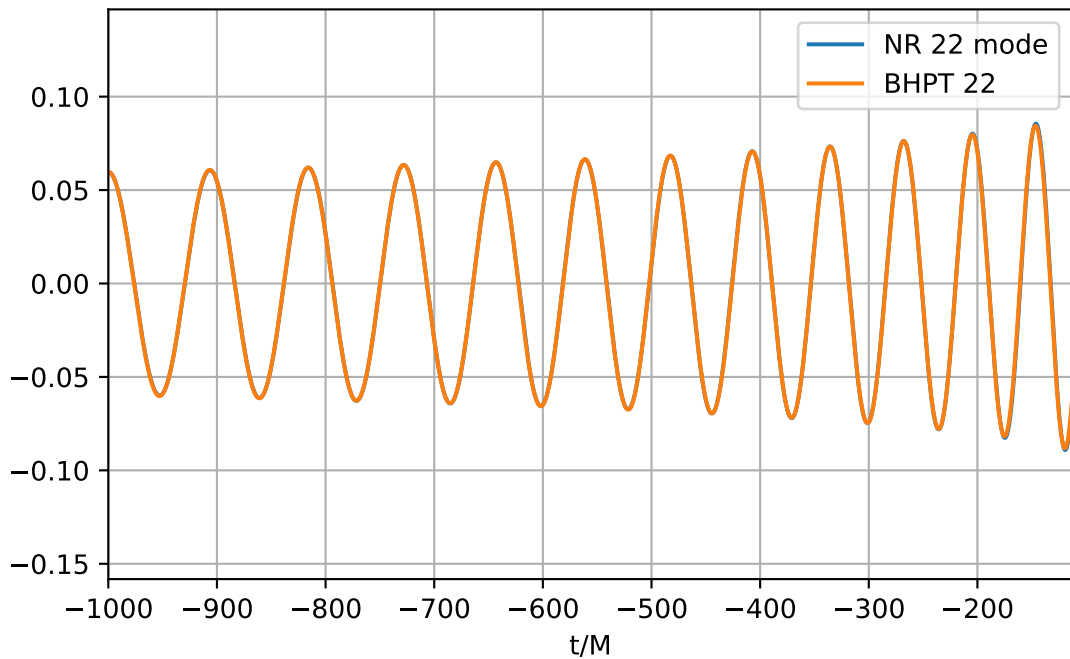
PN-opt q-dependent Agentic fit ( q = 8 ); \text{mathcal{E}} = 0.000107
