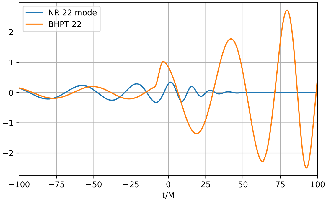
Physical-smooth q -dependent Agentic fit ( q = 2 )
