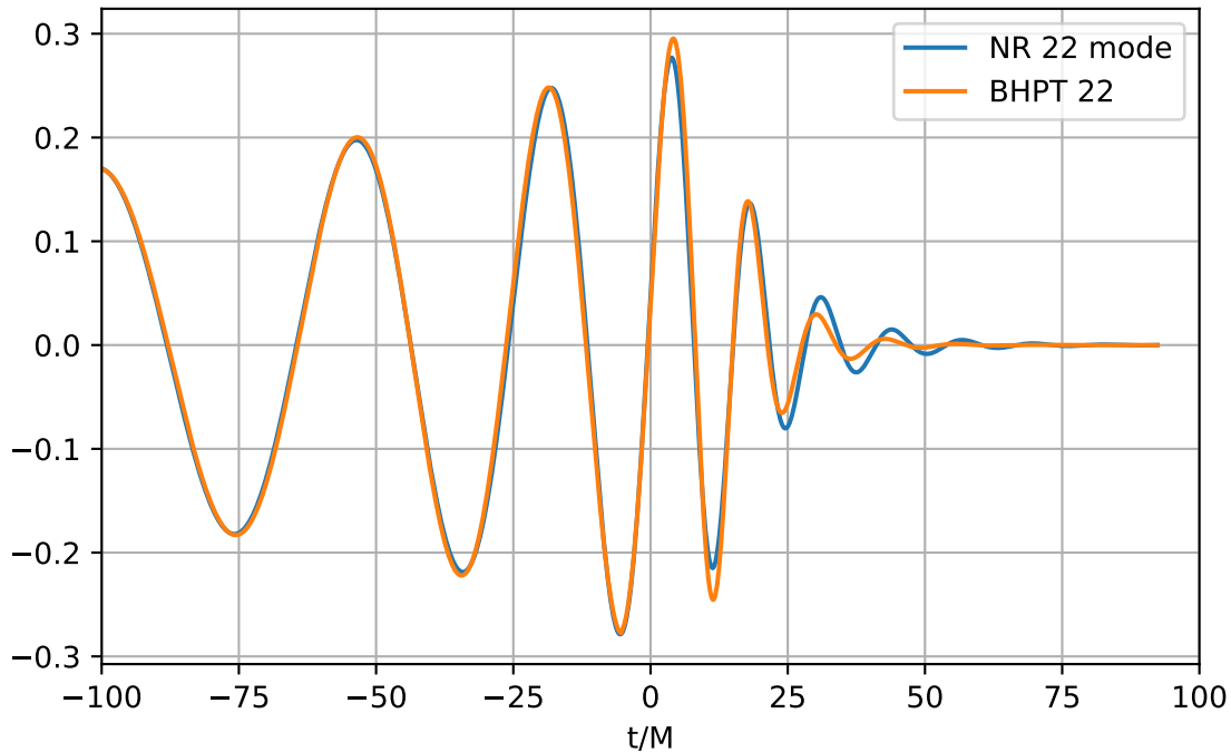
Physical-smooth q-dependent Agentic fit ( q = 3 )
