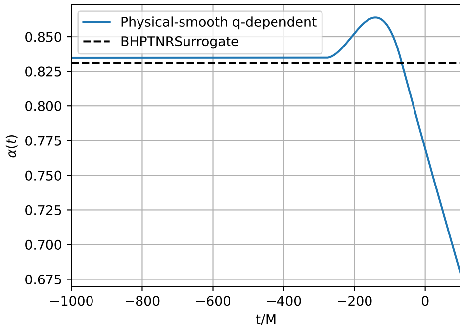
Physical-smooth q-dependent Agentic fit ( q = 6 )
