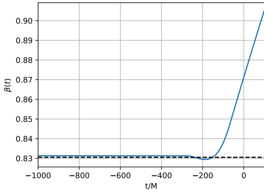
Physical-smooth q-dependent Agentic fit ( q = 6 )
