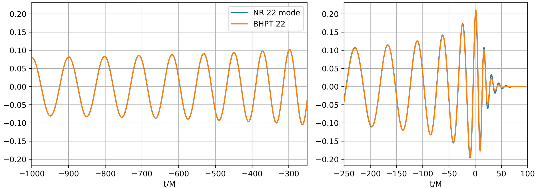
Reduced Stricter Smooth Agentic fit ( q = 5 )
