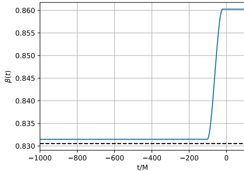
Two-constant q-dependent Agentic fit ( q = 6 )
