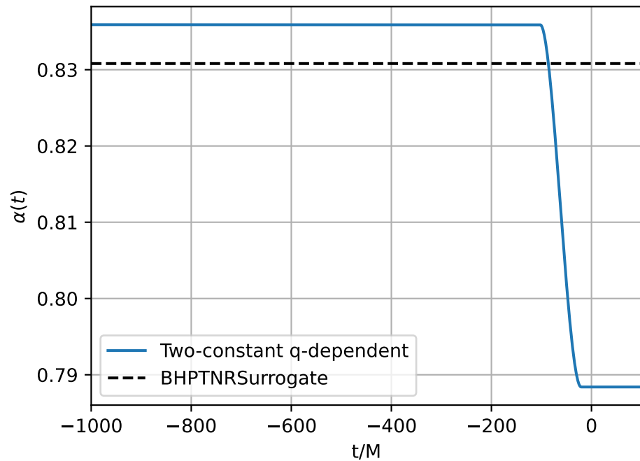
Two-constant q-dependent Agentic fit ( q = 6 )
