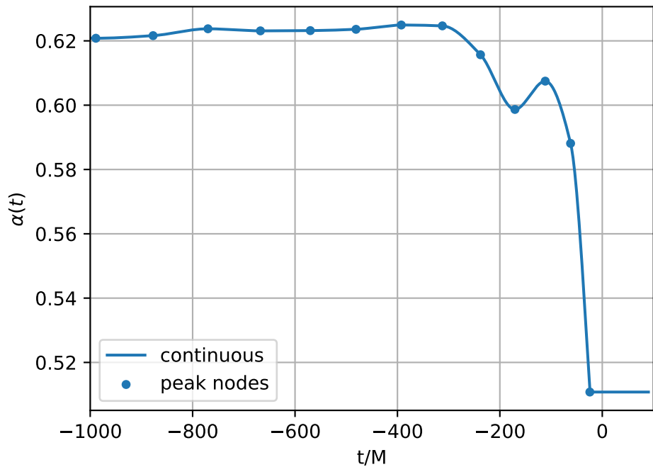
Waveform peak-ratio fit ( q = 2 )
