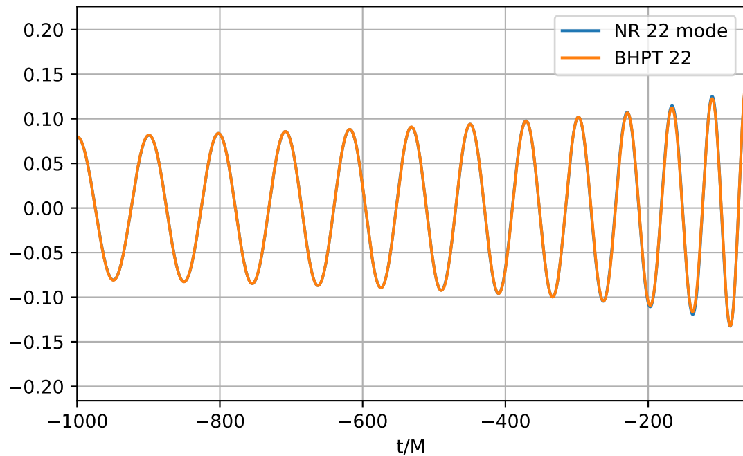
Creative smooth PN-loss fit ( q = 5 )
