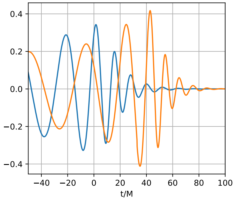
Creative PN-loss q-dep fit ( q = 2 ); \text{mathcal{E}} = 0.214
