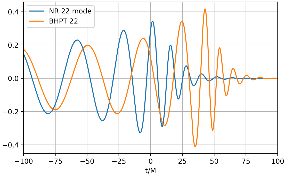
Creative PN-loss q-dep fit ( q = 2 )
