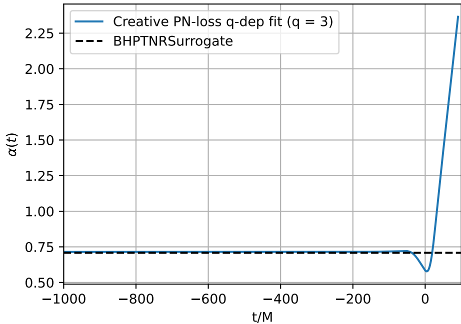
Creative PN-loss q-dep fit ( q = 3 )
