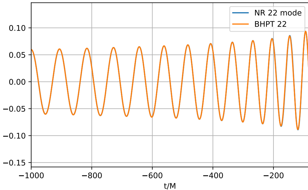
Creative PN-loss q-dep fit ( q = 8 ); \text{mathcal{E}} = 0.000145
