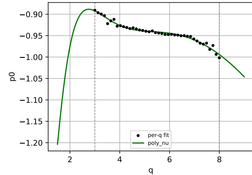
PN_opt_nu_Pade (poly_nu): parameter q-dependence (dashed = training edges; q < 3 is extrapolation)
