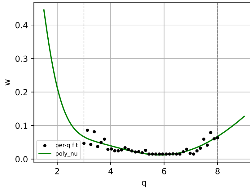
PN_opt_nu_Pade (poly_nu): parameter q-dependence (dashed = training edges; q < 3 is extrapolation)
