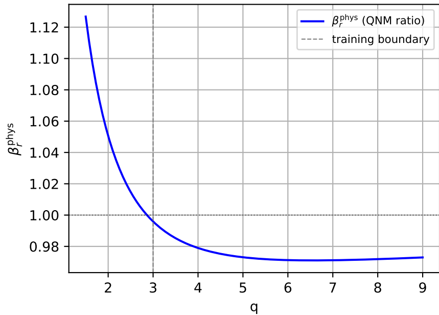
Physical QNM prediction
