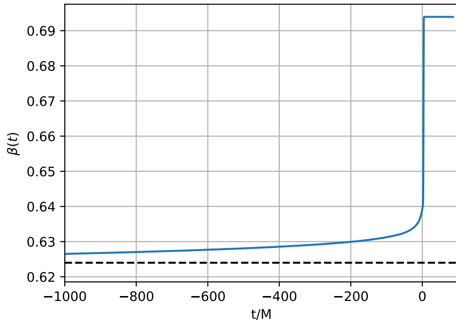
Remnant-partial q=2.0 [extrapolation]; \chi_f=0.623 \beta_{r\_phys}=1.051
