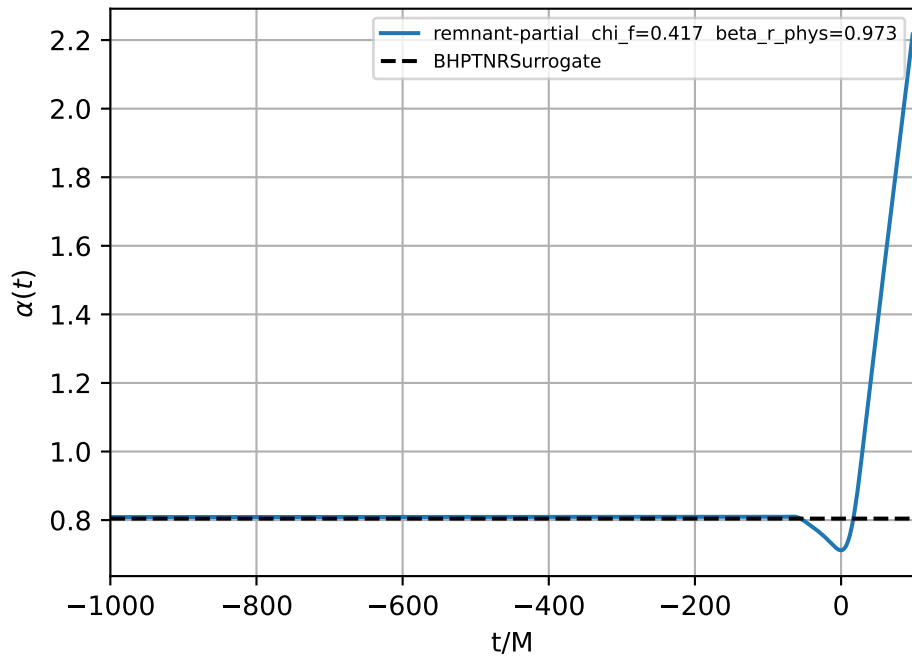
Remnant-partial q=5.0 ; \chi_f=0.417 \beta_r_{\text{phys}}=0.973
