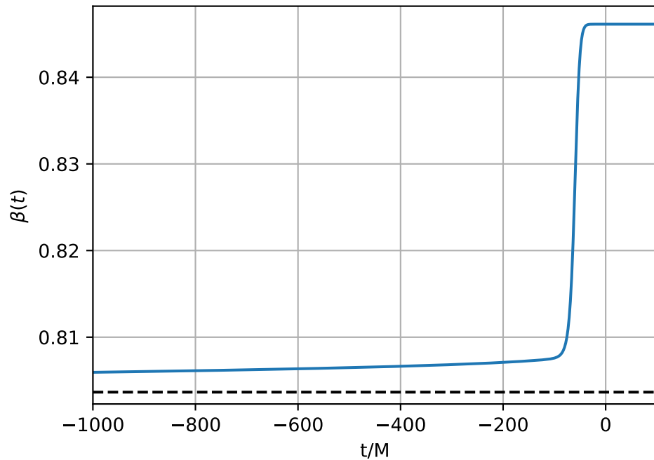
Remnant-partial q=5.0 ; \chi_f=0.417 \beta_r_{\text{phys}}=0.973
