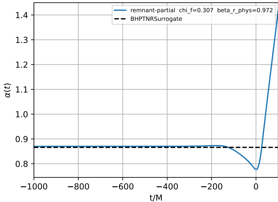
Remnant-partial q=8.0 ; \chi_f=0.307 \beta_{r\_phys}=0.972
