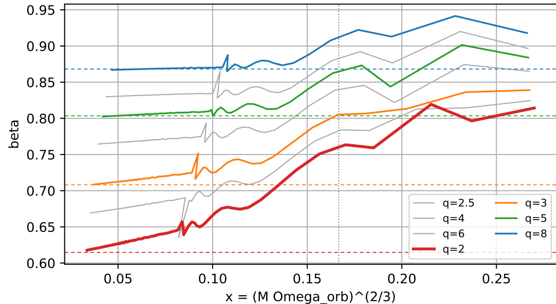
beta vs x (dashed: X1^{(6/5)} anchor)
