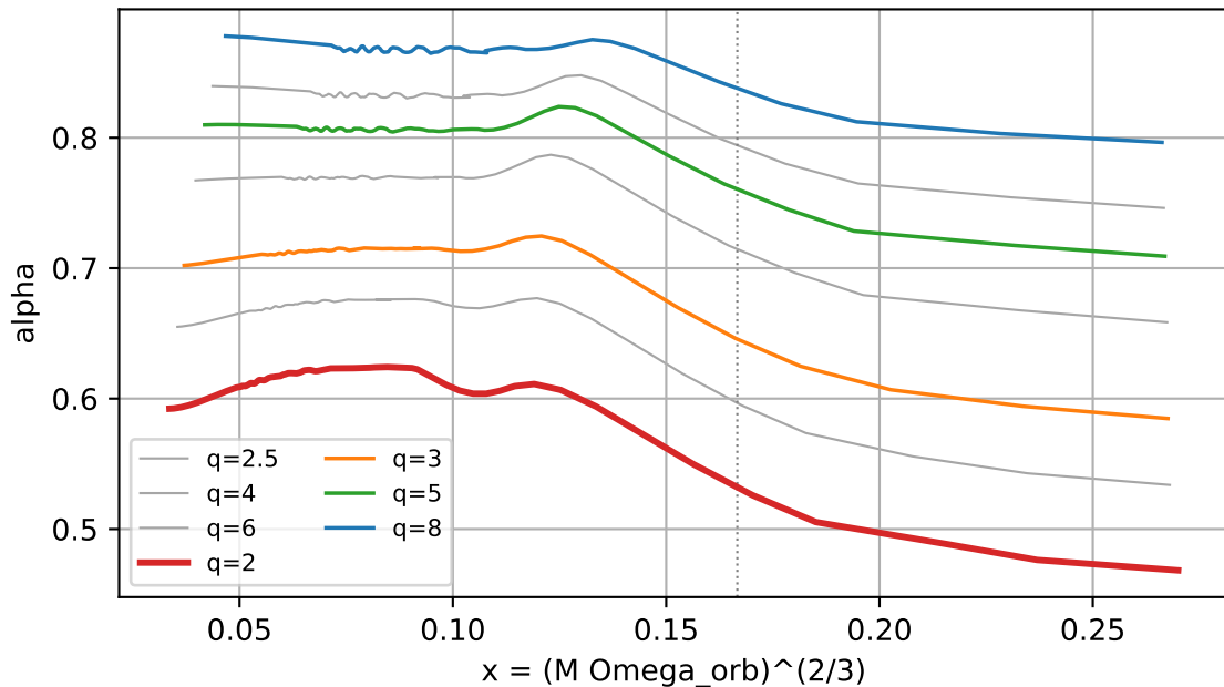
alpha vs x (parametric in t)
