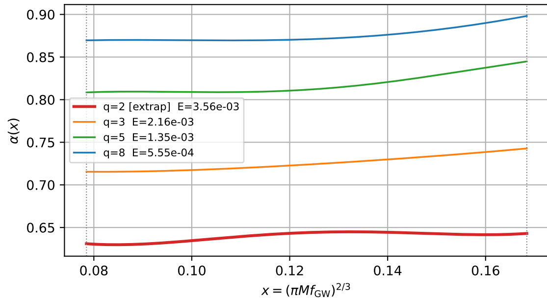
\alpha(x) — master
