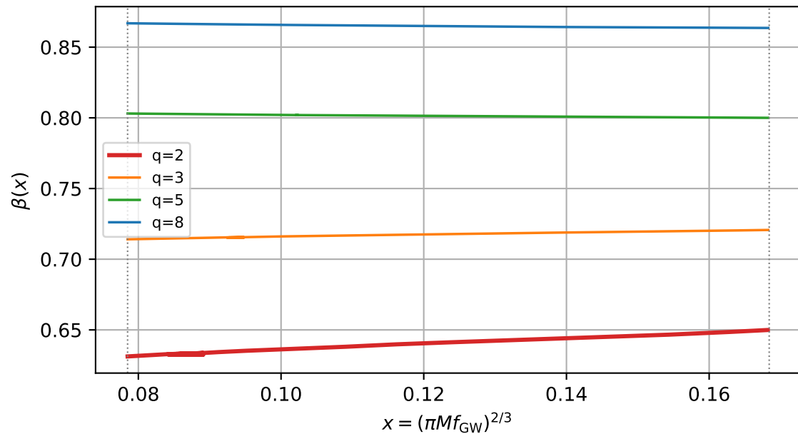
\beta(x) — master
