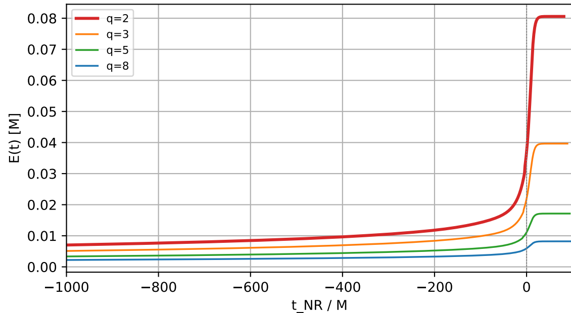
gw_remnant radiated energy
