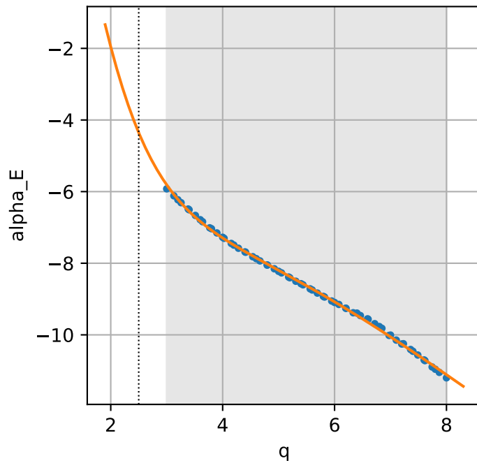
gw-remnant-energy: master coefficients vs q
