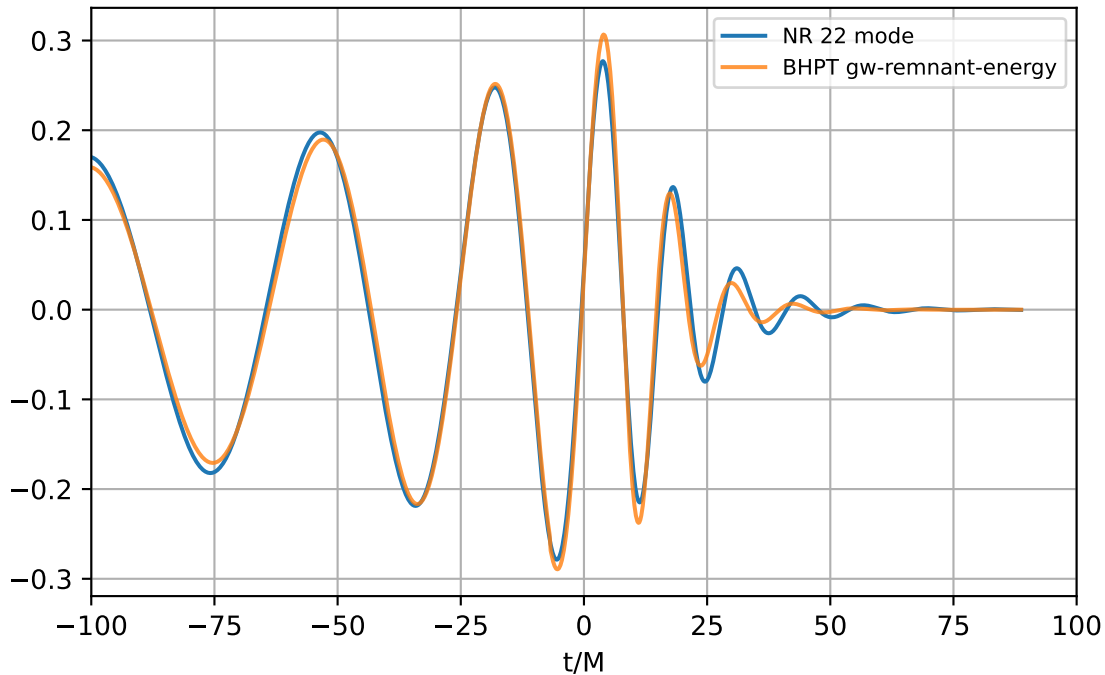
gw-remnant-energy q=3.0 ; \nu=0.1875
