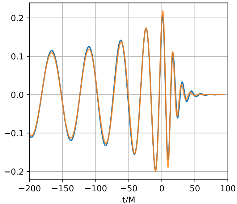
gw-remnant-energy q=5.0 ; \nu=0.1389 ; \text{mathcal{E}} = 0.0007
