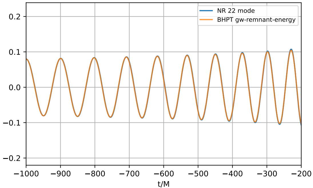
gw-remnant-energy q=5.0 ; \nu=0.1389 ; \text{mathcal{E}} = 0.0007
