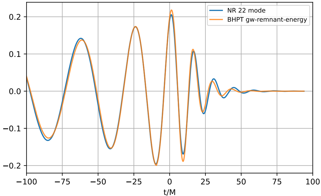
gw-remnant-energy q=5.0 ; \nu=0.1389
