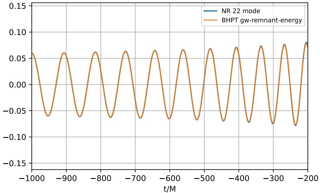
gw-remnant-energy q=8.0 ; \nu=0.0988 ; \text{mathcal{E}} = 0.000262
