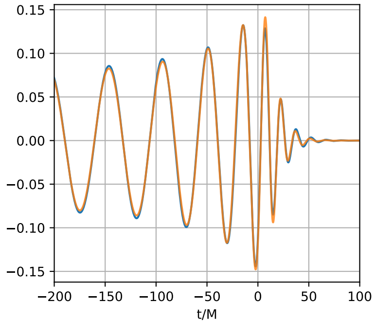
gw-remnant-energy q=8.0 ; \nu=0.0988 ; \text{mathcal{E}} = 0.000262
