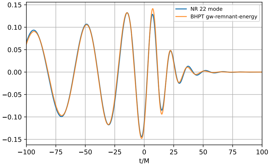
gw-remnant-energy q=8.0 ; \nu=0.0988
