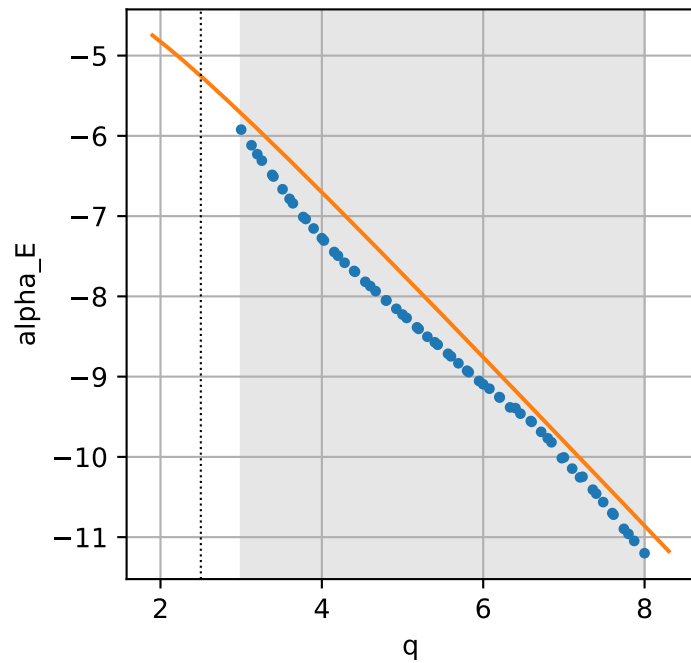
gwr-energy-anchored: master coefficients vs q
