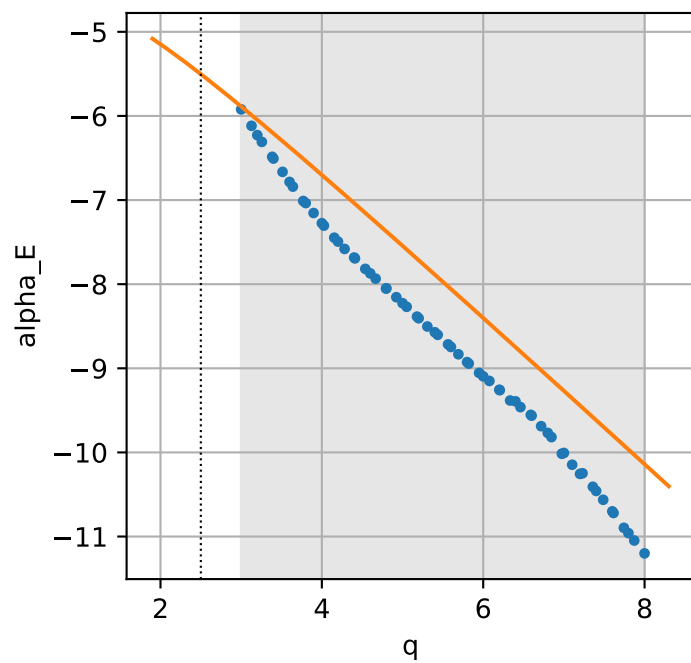
gwr-energy-stiff: master coefficients vs q
