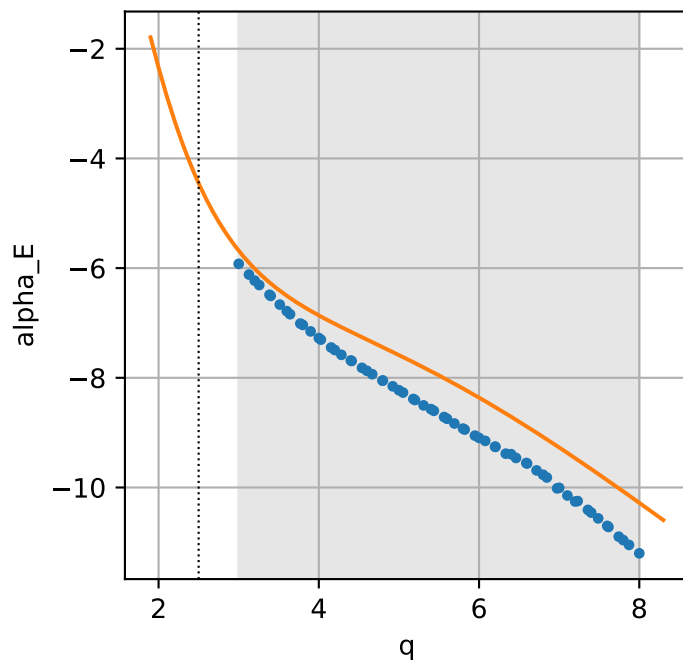
gwr-energy-global: master coefficients vs q
