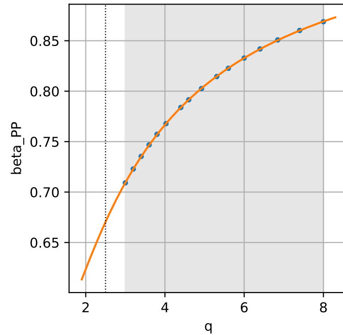
gwr-energy-flux: master coefficients vs q
