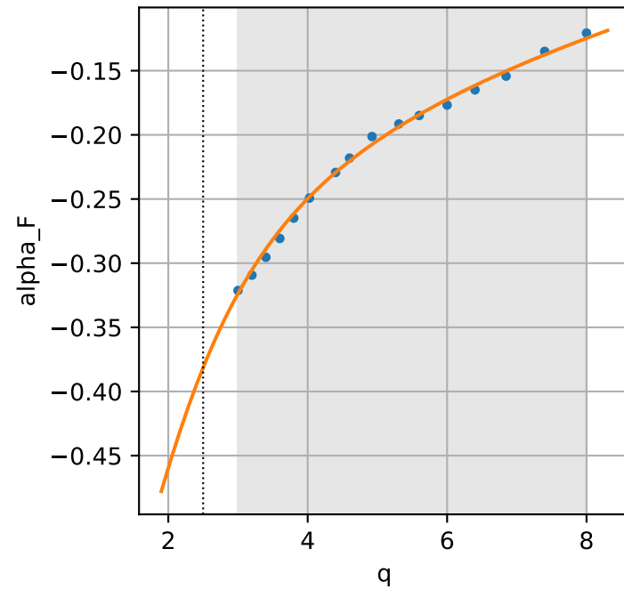
gwr-energy-flux: master coefficients vs q
