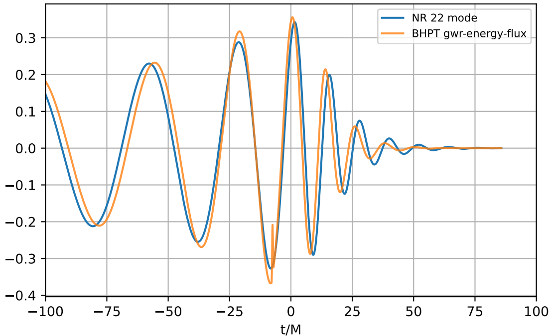
gwr-energy-flux q=2.0 [extrapolation]; nu=0.2222
