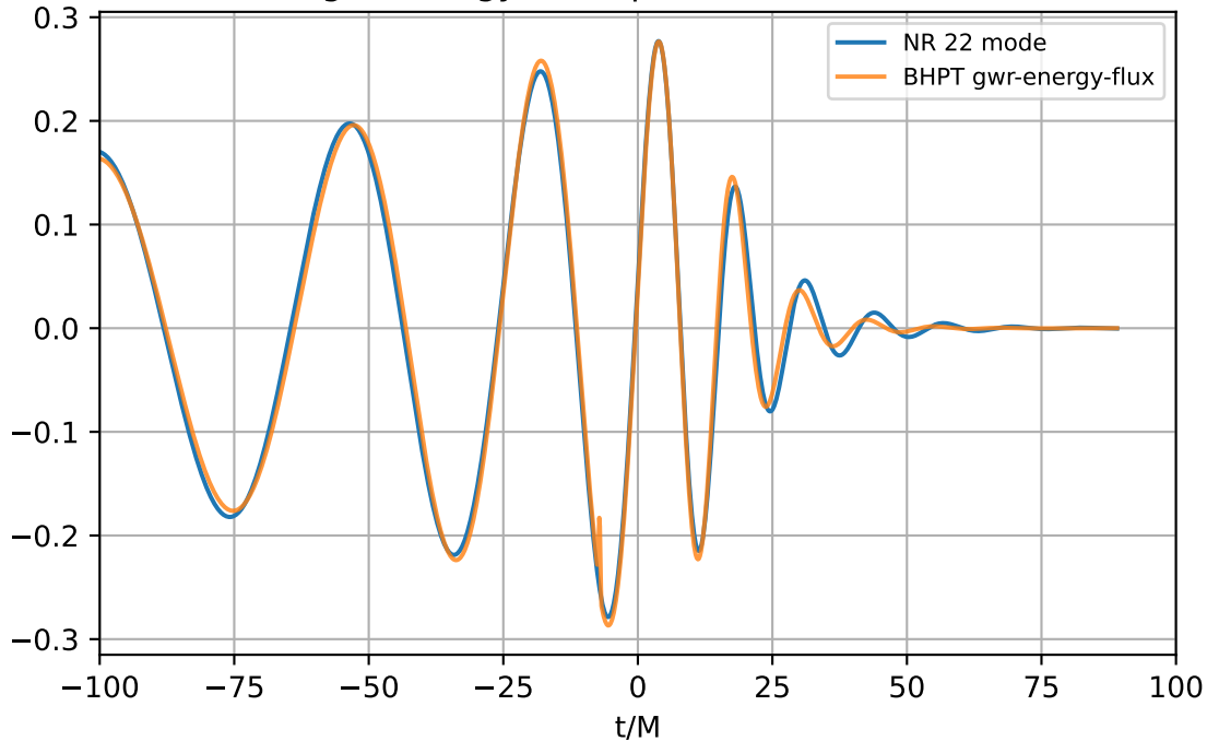
gwr-energy-flux q=3.0 ; \nu=0.1875
