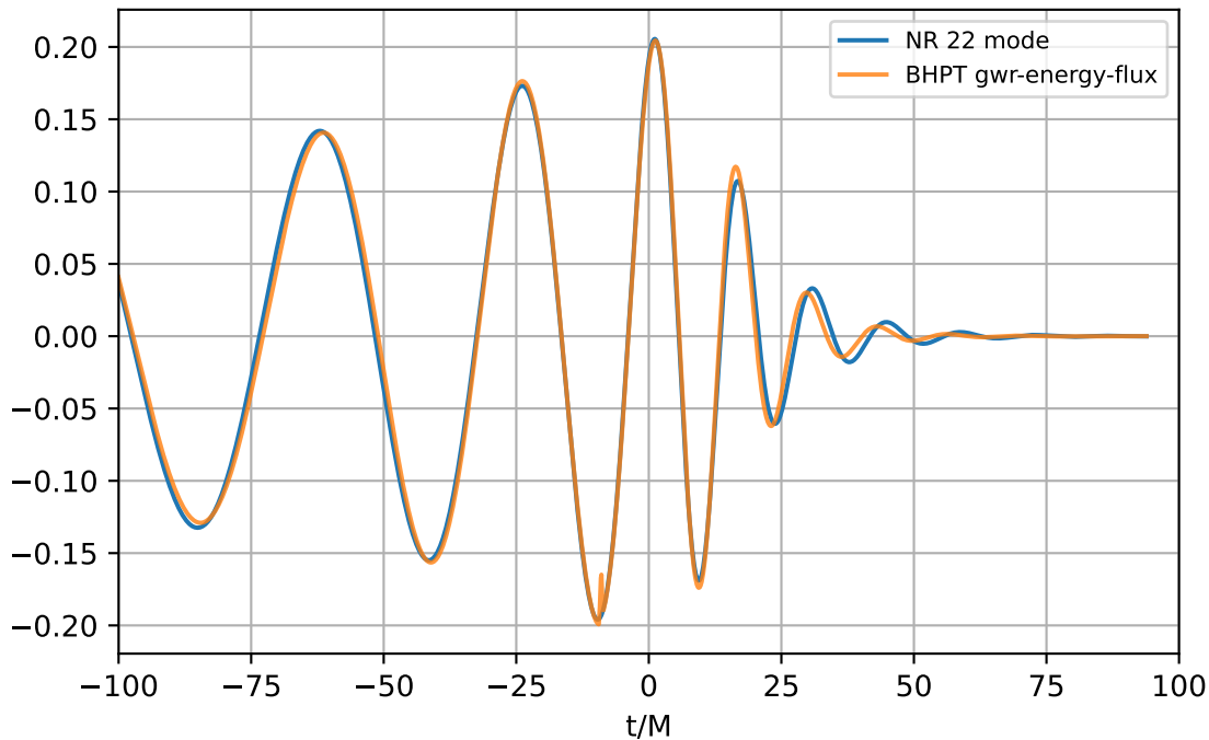
gwr-energy-flux q=5.0 ; \nu=0.1389
