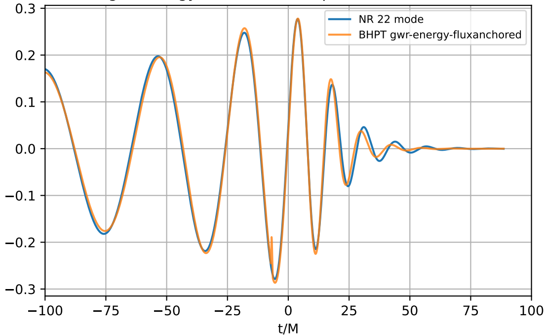
gwr-energy-fluxanchored q=3.0 ; \nu=0.1875
