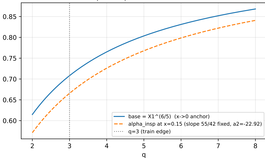
beta (inspiral anchor + remnant beta_r)
