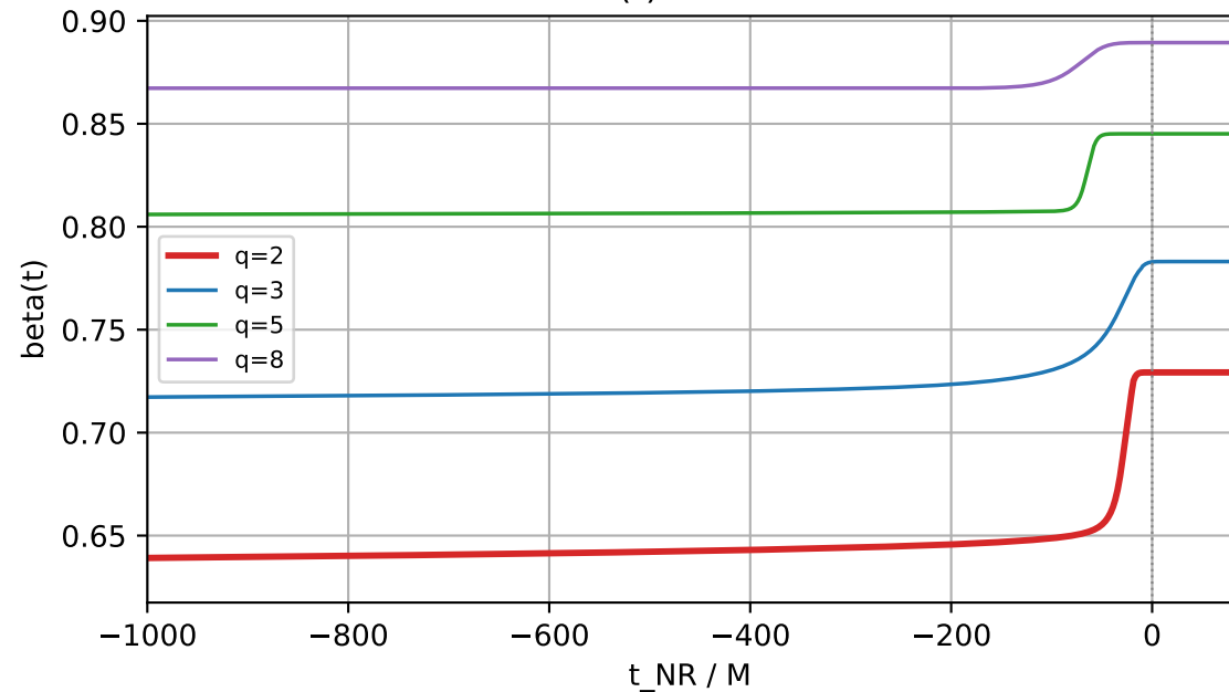
beta(t) — master
