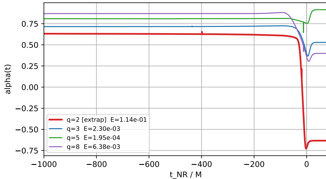
alpha(t) — master
