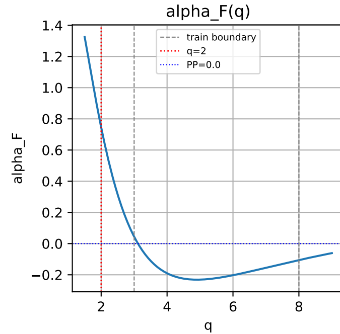
wf-nu-fluxes coupling parameters vs q
