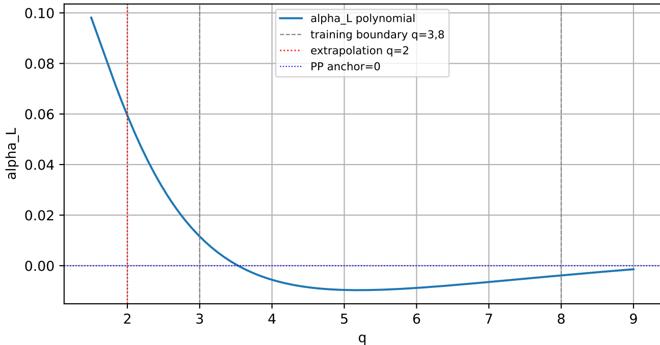
Inspiral alpha drift coefficient \alpha_L(q)
