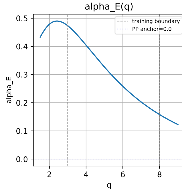
wf-nu-hybrid coupling parameters vs q (gray dashed = training boundary)
