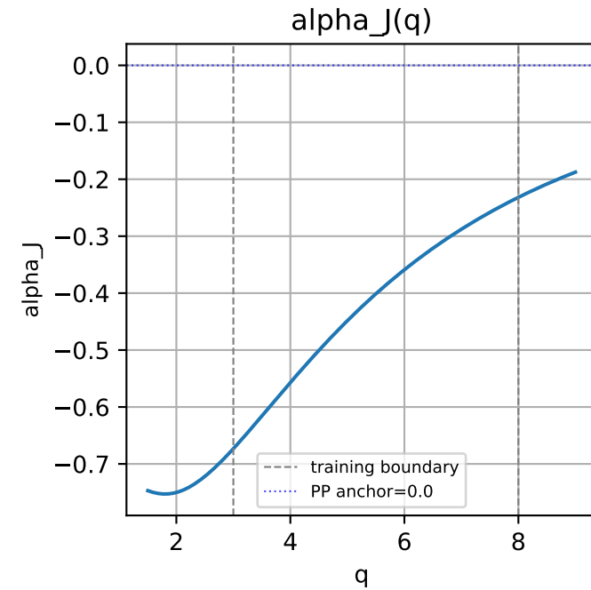
wf-nu-hybrid coupling parameters vs q (gray dashed = training boundary)
