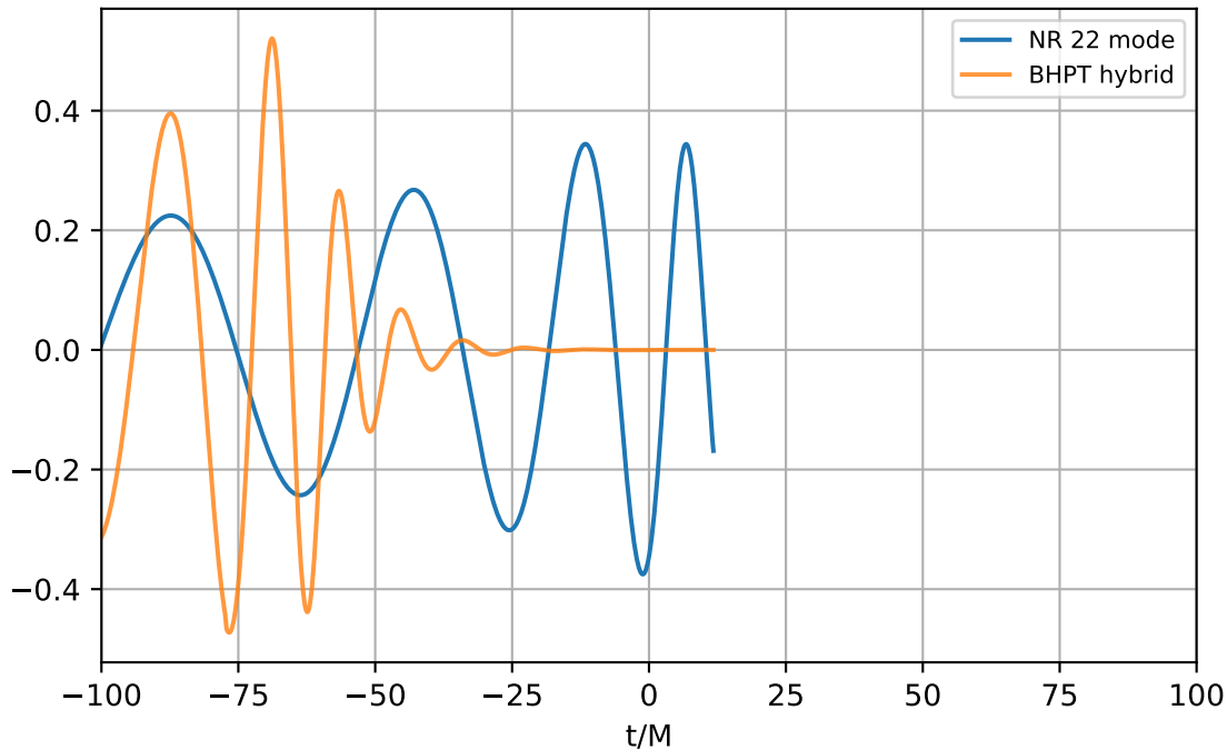
wf-nu-hybrid q=1.5 [extrapolation]; \nu=0.2400
