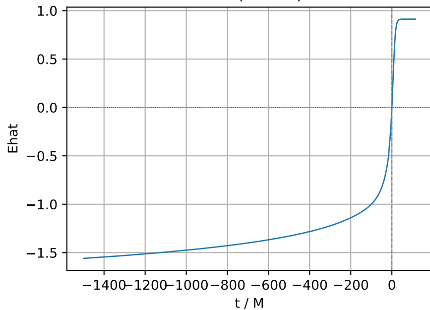
\hat{E} (wf flux)
