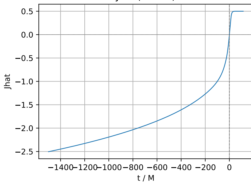
\hat{J} (wf flux)
