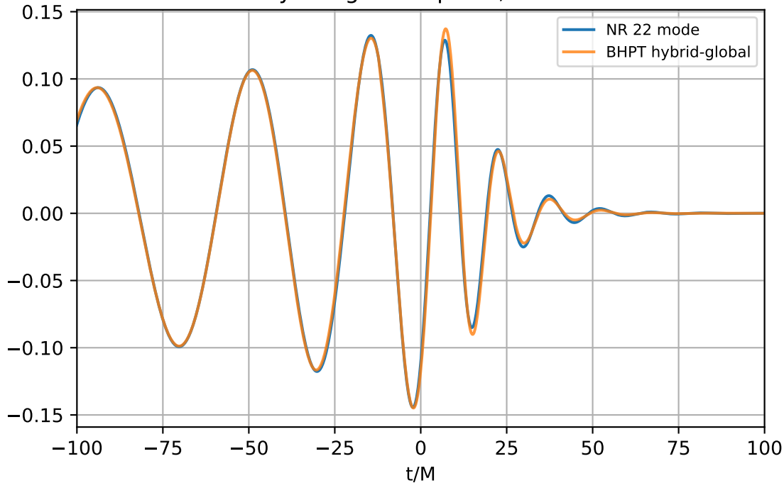
wf-nu-hybrid-global q=8.0 ; \nu=0.0988
