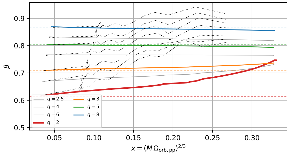
\beta vs x — MASTER (dashed: \chi_1^{6/5} )
