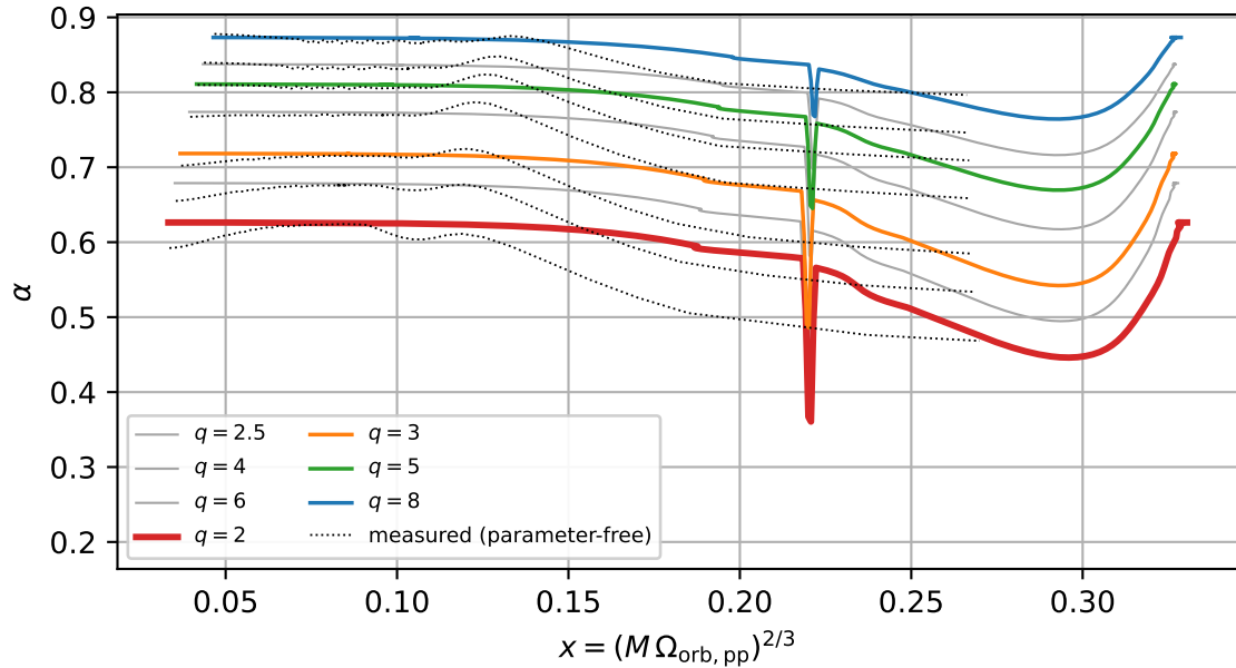
\alpha vs x — MASTER (colour) vs measurement (dotted)
