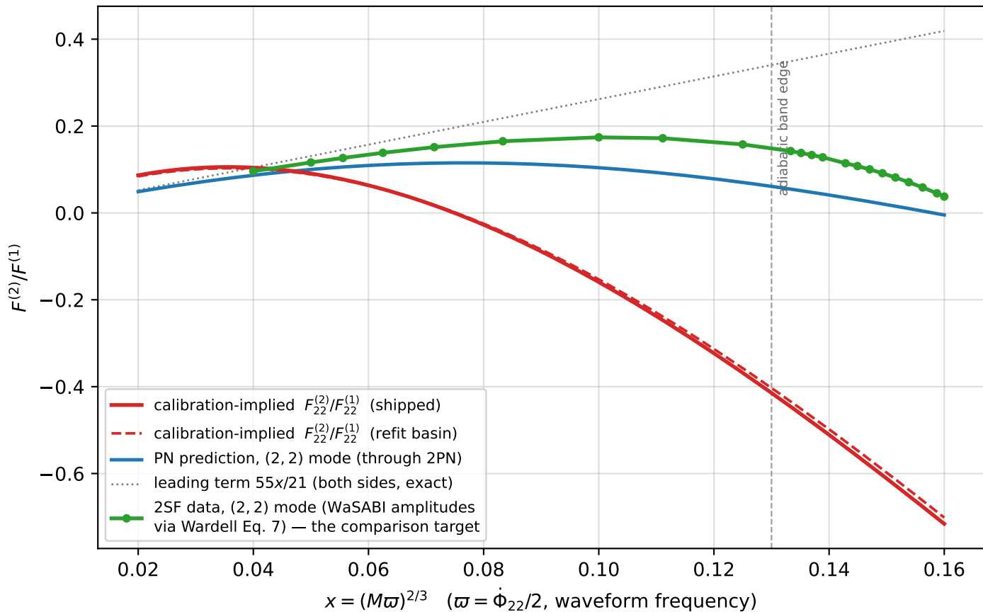
Second-order flux: calibration-implied vs self-force / PN
