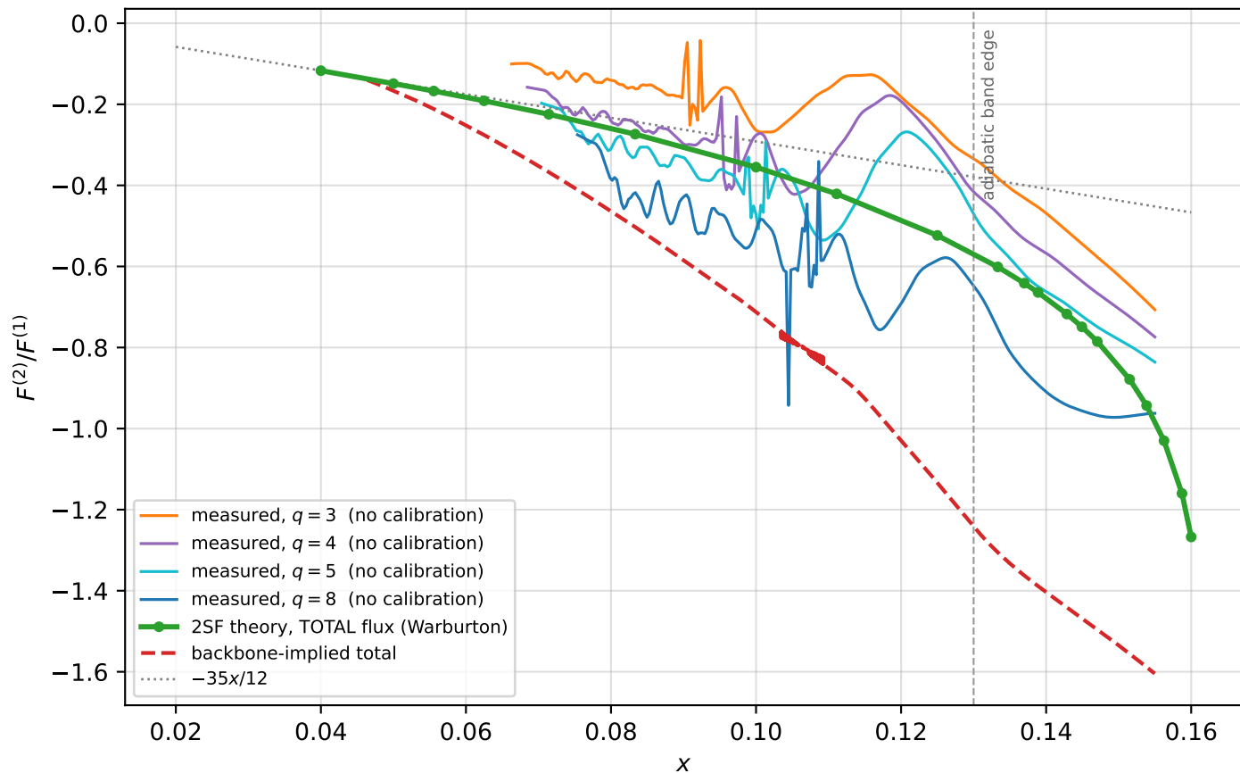
MEASURED TOTAL second-order flux ratio — no calibration
