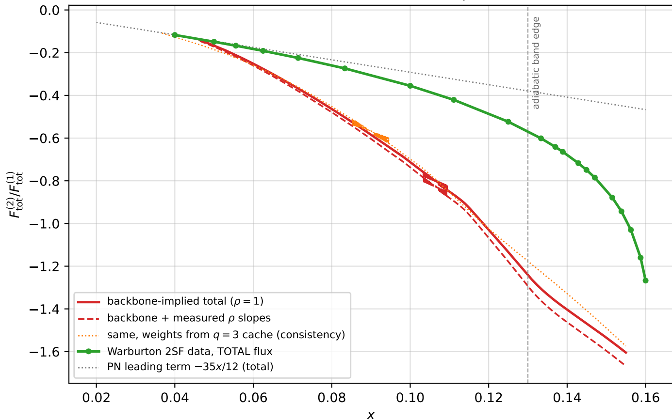
TOTAL second-order flux: hm-backbone-implied vs 2SF data
