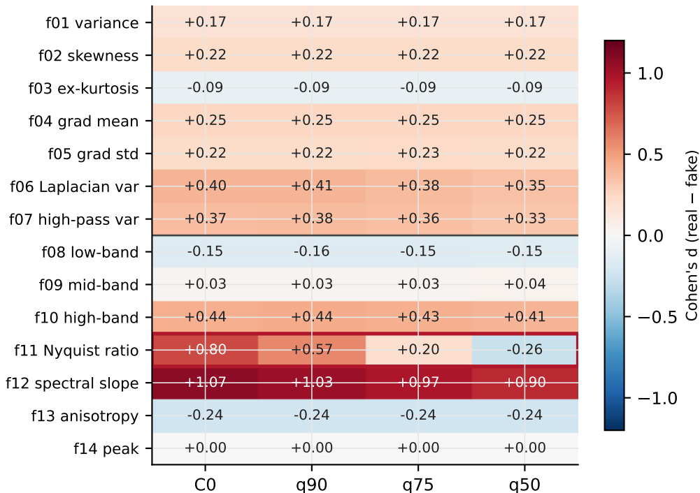
Per-feature effect size by JPEG condition (3,000 parents) rows 1-7 pixel-pattern, 8-14 frequency; positive = real higher; red outline = the f11 sign flip
