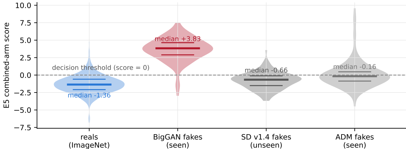
E5 (unseen SD v1.4 in test, JPEG q75): combined-arm score distributions
